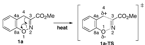
FIGURE 3. Electron shifts in the retro-Diels–Alder reaction of 4 H -1,2-benzoxazine ( 1a ).
