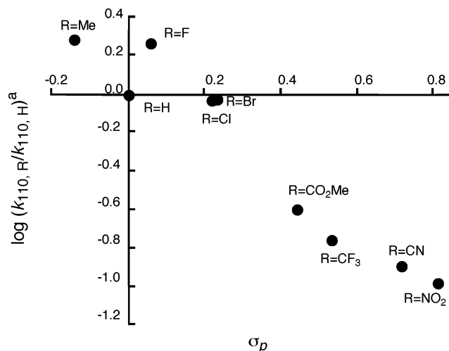
FIGURE 4. Correlation between the relative reaction rate constants ( k_{110} , the reaction rate constant of the retro-Diels–Alder reaction in toluene at 110 °C) and Hammett \sigma_p . 15
