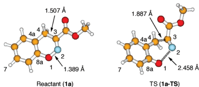
FIGURE 1. Calculated structures of reactant and transition state in the retro-Diels–Alder reaction of unsubstituted 4 H -1,2-benzoxazine ( 1a ).
