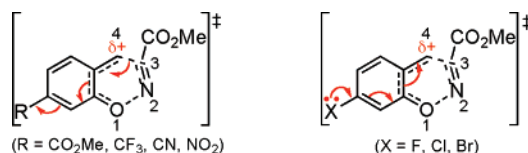
FIGURE 5. Resonance destabilization (left)/stabilization (right) of the transition state arising from the substituent at C 7 .
