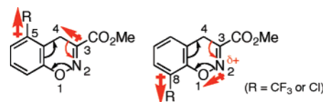
FIGURE 6. Deceleration (left) and acceleration (right) of C 3 –C 4 bond cleavage.
