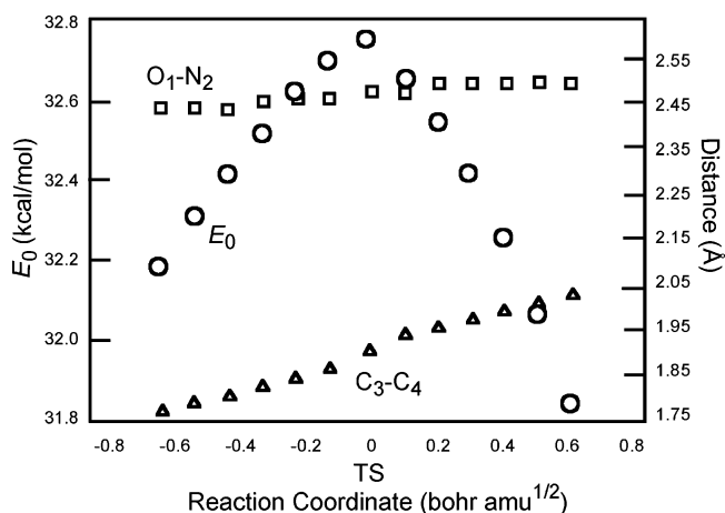
FIGURE 2. Increases of C 3 –C 4 and O 1 –N 2 bond lengths in the vicinity of the transition state (B3LYP/6-31+G(d,p) level).
